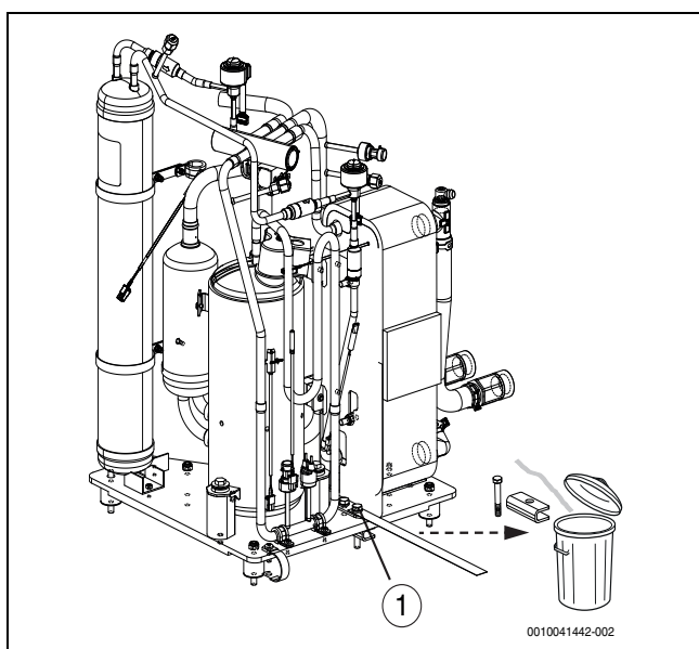
Fig. 33 Transportfitting
