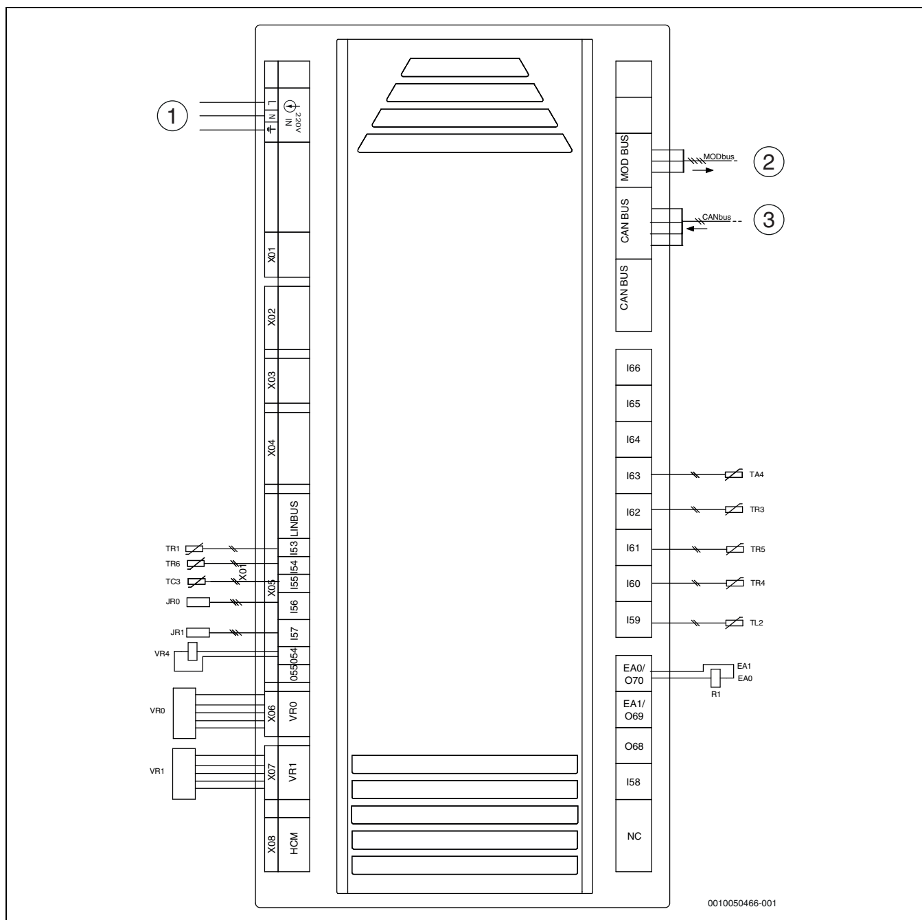
Fig. 48 Strømdiagram XCU-SRH (XCU-HP)
